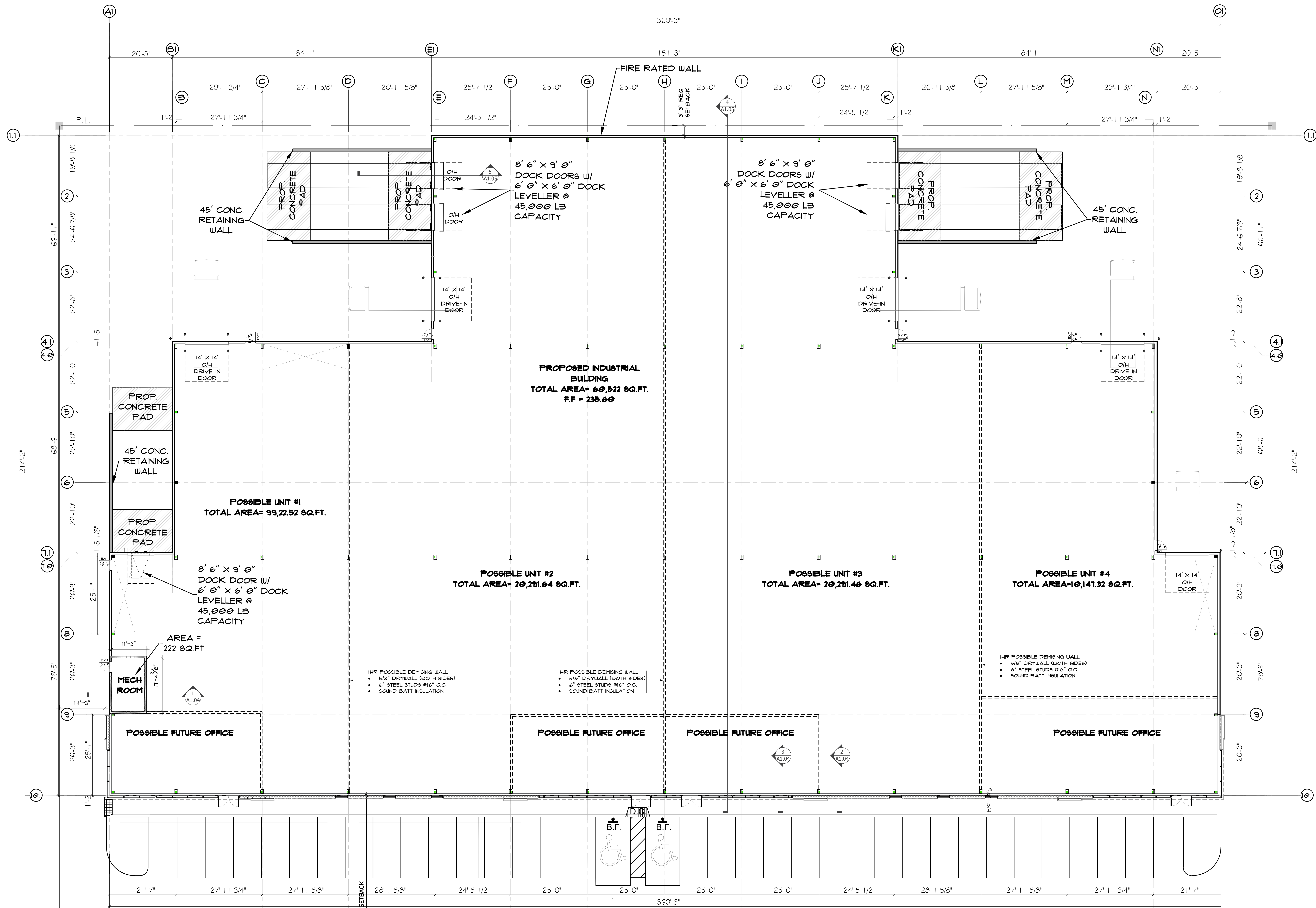
1 FLOOR PLAN A2.1 SCALE: 1/16"=1'
